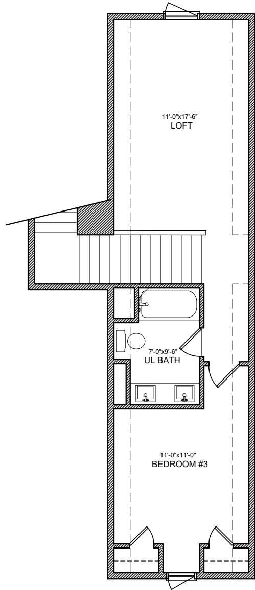
UPPER LEVEL PLAN
