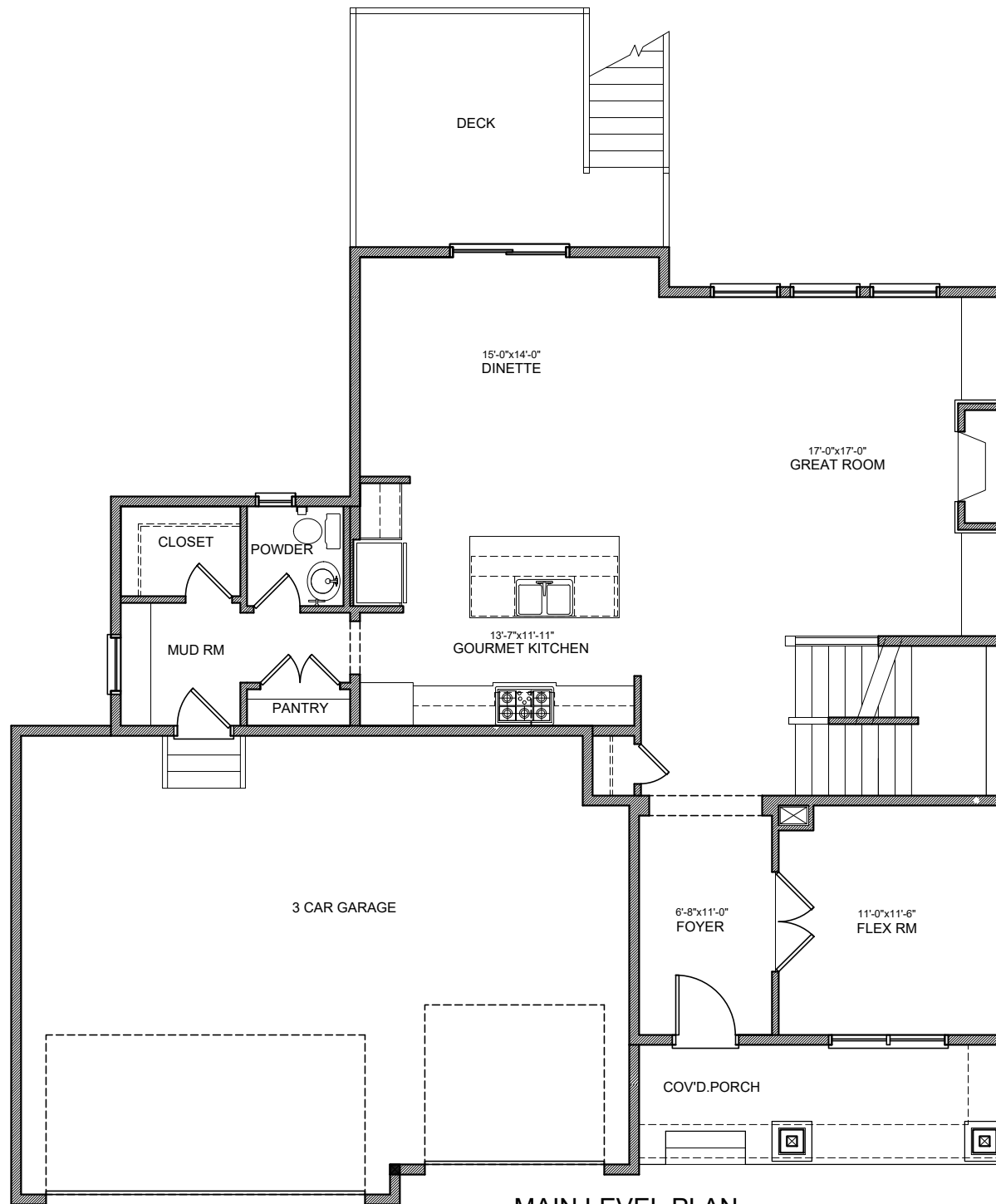
MAIN LEVEL PLAN
